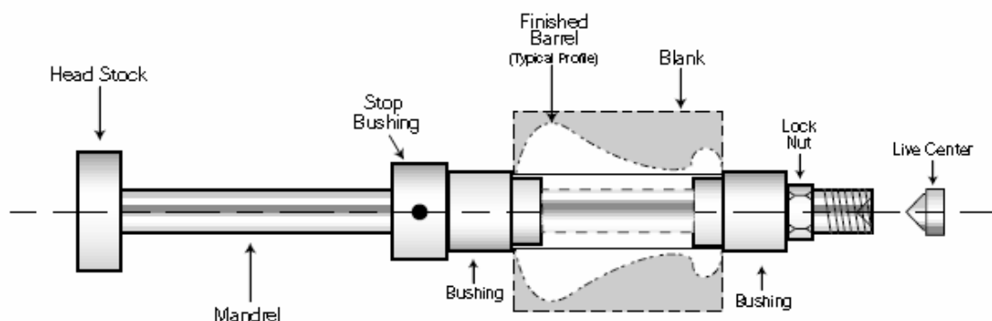
Diagram B / Mounting Parts on the Mandrel
